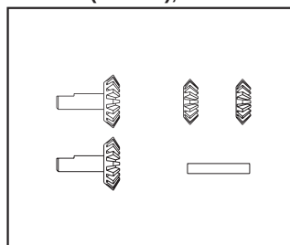
PD2118 DIFF. BEVEL GEAR, ZT&ZK
