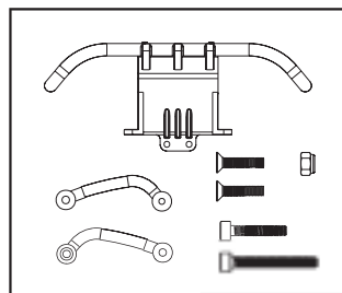
PD2114 RR BUMPER SET, ZK
