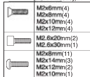
PD2179 SCREW KIT, ZK & ZT
